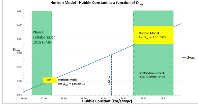
FIG. 2. Horizon Model (HM) values of the Hubble constant as a function of \Omega_{vac} . With \Omega_{vac} = \Omega = 1.00 \pm 0.01 , the HM value for H ( 67.87 \pm 0.38 ) agrees very well with the Planck collaboration measurement. The HM values for H are in agreement with the SH0ES team measurement if \Omega_{vac} = 1.16 \pm 0.03 . For a Hubble time of 13.8 Gyr, \Omega_{vac} = 1.094 .
