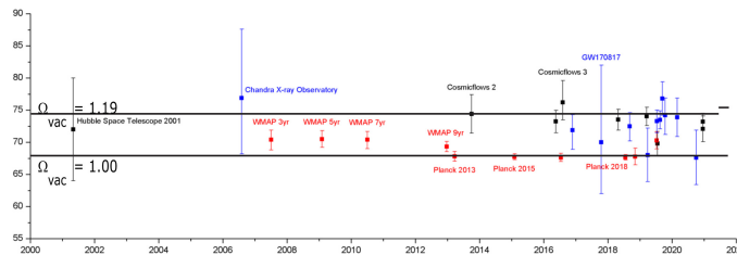
FIG. 3. Estimates of H_0 , 2001 – 2020. Estimates in black represent calibrated distance ladder measurements; red represents early universe CMB/BAO with \Lambda CDM Parameters; blue are other techniques. The solid lines are the HM values for H_0 = H_{vac}(\Omega_{vac}) .
