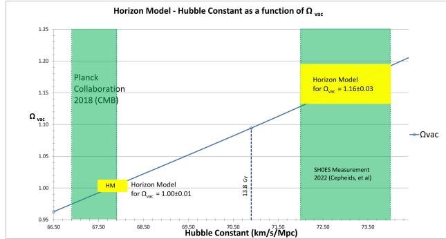
FIG. 2. Horizon Model (HM) values of the Hubble constant as a function of \Omega_{vac} . With \Omega_{vac} = \Omega = 1.00 \pm 0.01 , the HM value for H ( 67.87 \pm 0.38 ) agrees very well with the Planck collaboration measurement. The HM values for H are in agreement with the SH0ES team measurement if \Omega_{vac} = 1.16 \pm 0.03 . For a Hubble time of 13.8 Gyr, \Omega_{vac} = 1.094 .
